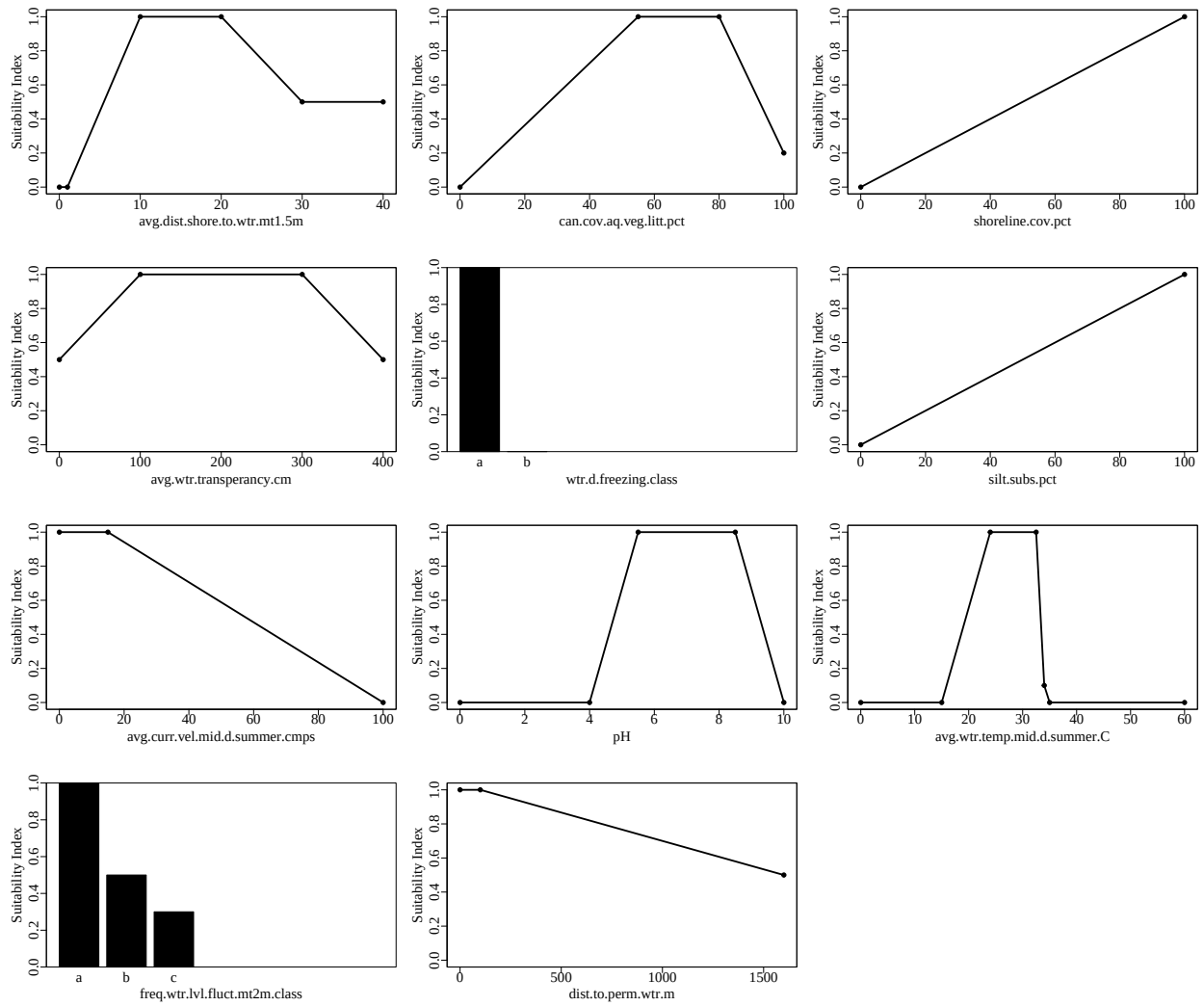
Figure 1. Suitability index graphs for variables included in the bullfrog model in ecores.
